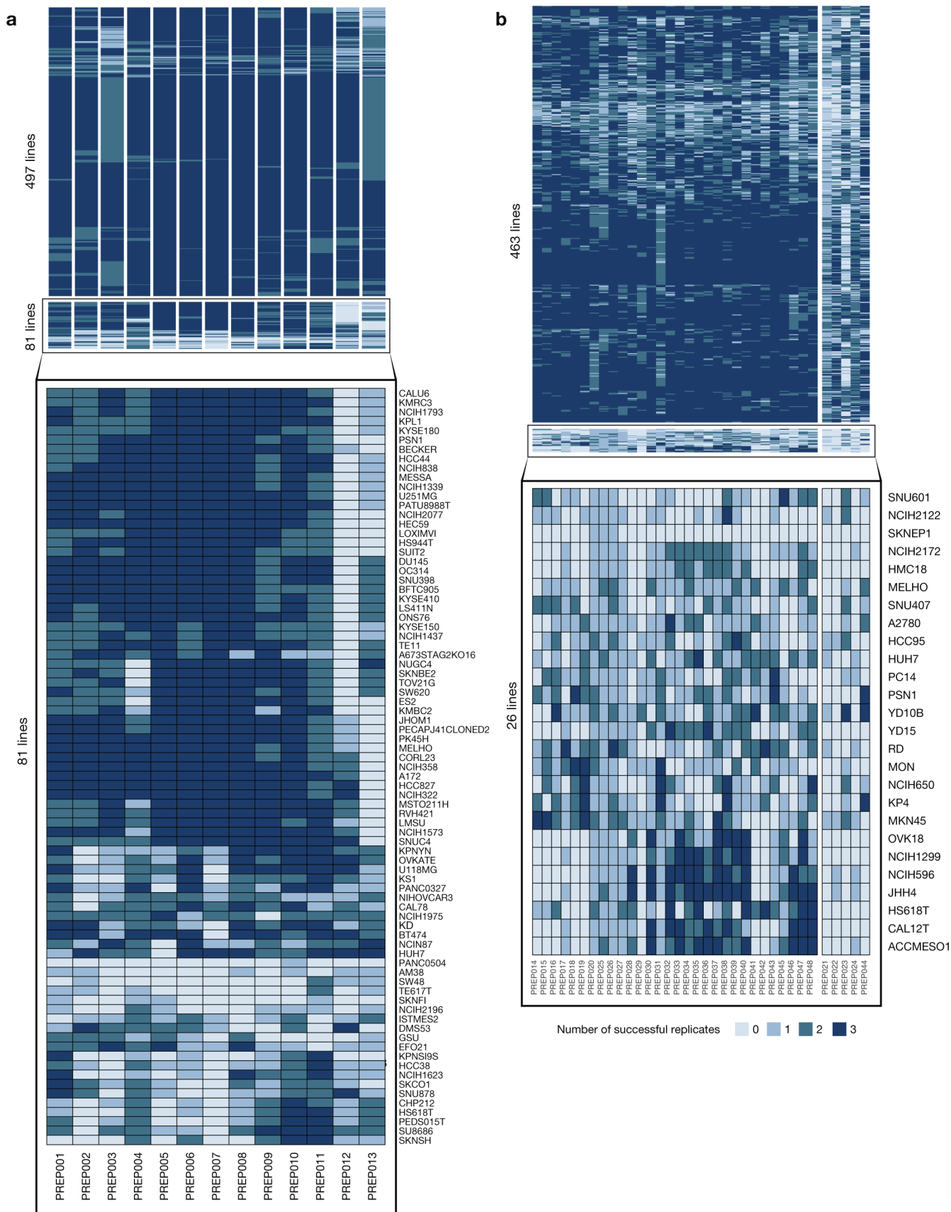
Extended Data Fig. 4 | Number of well replicates passing QC in the PRISM screens. a , Number of individual cell assay well replicates (max n=3) that pass QC filters in the primary screen, grouped by compound plate and cell line quality. 86% (497 out of 578) of the cell lines have at least one passing replicate for all compound plates. Identity of cell lines with lower quality data are listed at the bottom. b , Number of individual cell assay well replicates (max n=3) that pass QC filters in the secondary screen. 95% (463 out of 489) of cell lines have at least 1 passing replicate on at least 85% (30 out of 35) of the compound plates.
