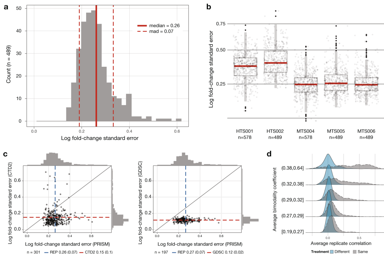
Extended Data Fig. 6 | PRISM Repurposing noise quantification. a , Cell line standard error estimates across vehicle-treated wells on PRISM plates treated with DMSO (n = 489 cell lines). Log fold change standard errors are estimated for each cell line using DMSO-only plates included in the MTS006 screen (n = 384 × 3 replicate wells for each cell line). b , Comparison of standard error estimates across screens. The error estimate calculation is repeated for each screen using DMSO wells on standard compound plates (n = 32 replicate wells per plate), except for MTS006, which uses DMSO-only plates (n = 384 replicate wells per plate). Higher noise levels are observed in the initial high-throughput screens HTS001 (n = 578 cell lines) and HTS002 (n = 489 cell lines) compared with the medium-throughput screens MTS004 (n = 578 cell lines), MTS005 (n = 489 cell lines), and MTS006 (n = 489 cell lines). Upper box limits, center lines, and lower box limits correspond to 75 th , 50 th , and 25 th percentiles, respectively. Whiskers extend from the box limits to the most extreme value up to 1.5 IQR from the median. All cell lines are depicted as points, regardless of outlier status. c , Comparison of estimated standard error of vehicle control wells between high-throughput pharmacogenomic datasets. The average standard error across cell lines (n = 301 cell lines for PRISM versus CTD2 and n = 197 for PRISM versus GDSC) is indicated by dashed lines with standard deviation in parentheses. d , Relationship between drug selectivity and replicate reproducibility in PRISM. Average Pearson correlation between replicates for each compound, dose, and screen combination is stratified by mean bimodality coefficient. For comparison, the null distribution for randomly paired compounds is shown in blue.
